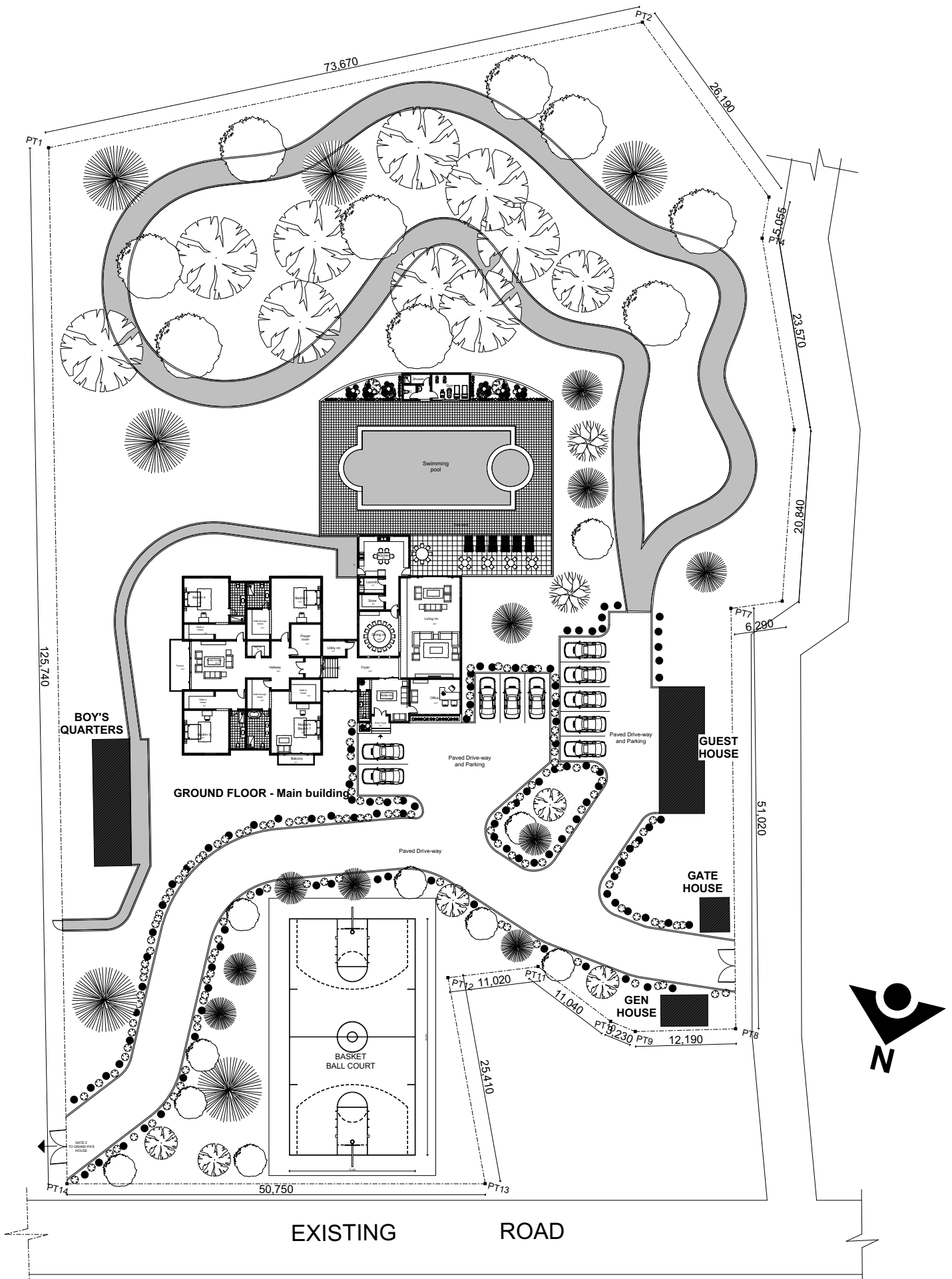
SITE PLAN REV 2
